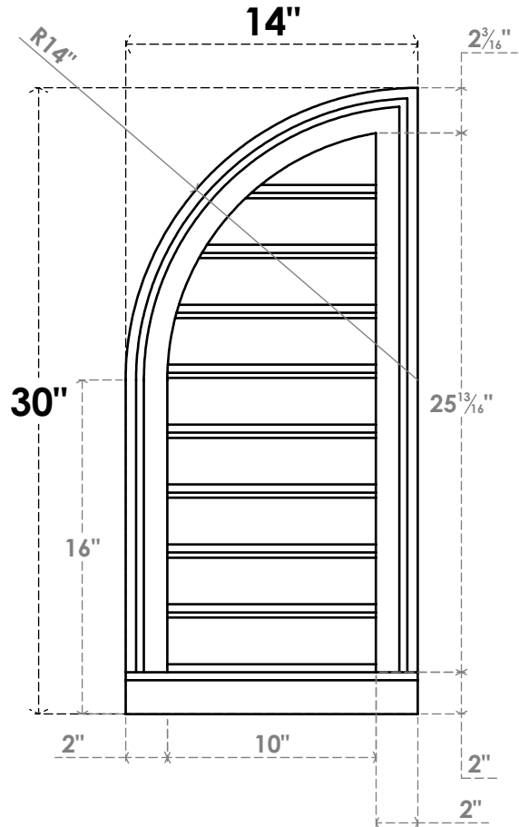
FRONT
